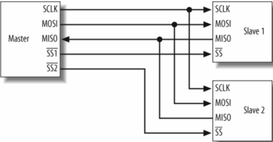
Figure 13-3. Example SPI bus structure
