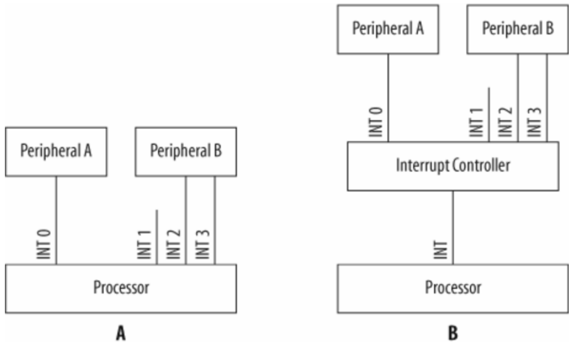
Figure 8-1. Interrupt wiring
