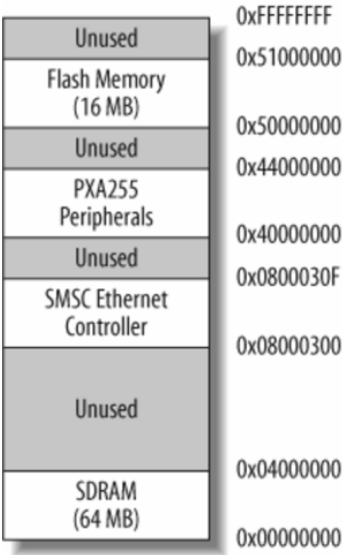
Figure 2-6. Memory map for the Arcom board
